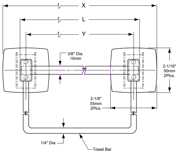
STANDARD STOCK SIZES
